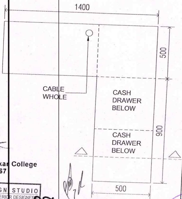
PLAN OF CASH COUNTER
