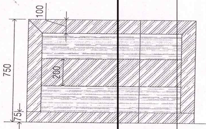
ELEVATION OF TABLE-1
