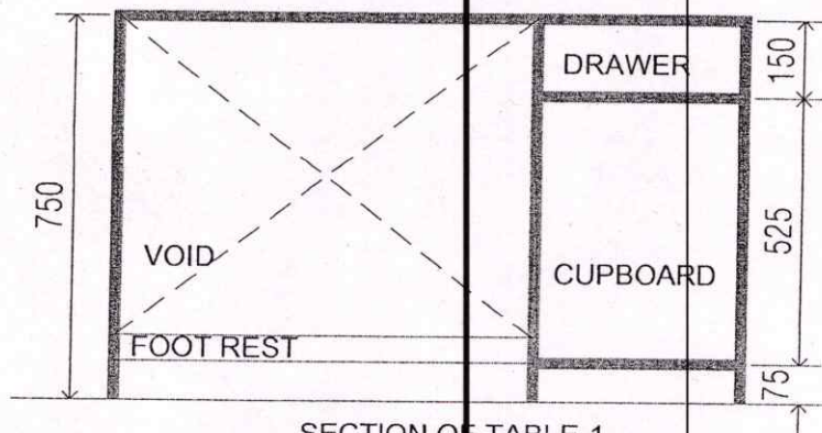
SECTION OF TABLE-1
